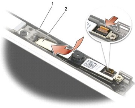
1 camera/microphone assembly 2 notch on display cover
